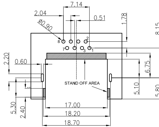
PCBLAYOUT TOP VIEW TOL:±0.05(THICKNESS=1.60)
